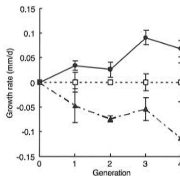
Fig. 4. Rates of larval growth in small- (closed circles) and large-harvested (closed triangles) populations relative to random-harvested controls (open squares). Each generation, the rate of larval growth at 21°C was measured by stocking 30 15-day-old larvae from each population into 19-liter polyethylene containers supplied twice daily with live Artemia nauplii ad libitum until age 45 days. There were three to four replicates per generation and line. Initial mean length was estimated from 10 to 15 fish killed at the outset of each trial. Growth rate of each replicate was calculated as [(\text{mean length on day 45}) - (\text{mean length on day 15})]/30 . The deviations of each of the treatment means from the mean growth rate of the controls are plotted. Vertical lines represent the range of values for the two replicate populations of each treatment. Regression analyses showed that the rate of larval growth increased significantly with generation in the small-harvested lines (slope = 0.79, SE = 0.21, P = 0.006 ) and decreased significantly with generation in the large-size-harvested lines (slope = -0.80, SE = 0.21, P = 0.006 ).
