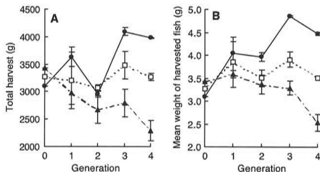
Fig. 1. Trends in average total weight harvested (A) and mean weight of harvested individuals (B) across multiple generations of size-selective exploitation. Closed circles represent small-harvested lines, open squares are the random-harvested lines, and closed triangles are the large-harvested lines. Each datum is the mean, and the vertical lines show the range of two replicate populations per treatment.
