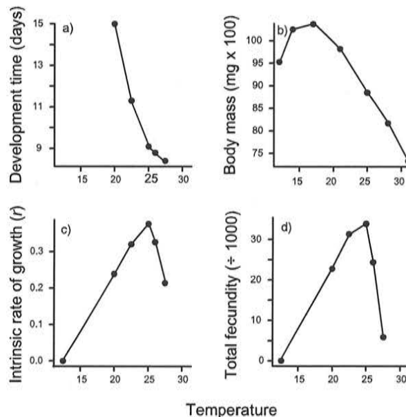
Fig. 5. Effects of rearing temperature on development time, body mass, r and R_0 for Drosophila melanogaster . Data from Karan et al. (1998) and Siddiqui and Barlow (1972).
